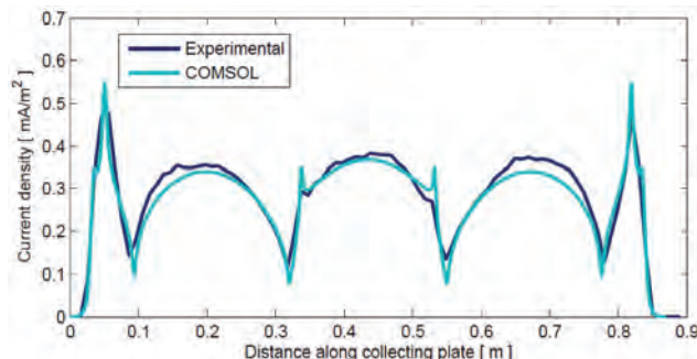
FIGURE 5: Current distribution entering the collecting plates, according to experimental measurement and numerical simulation. The “current spikes” are due to the profiling of the plate. The average current density corresponds to 250 \mu\text{A}/\text{m}^2 .
