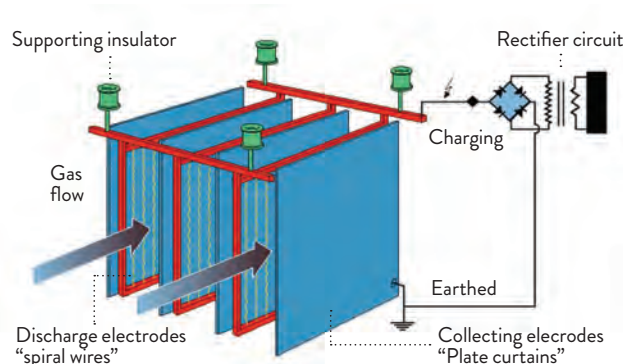
FIGURE 2: Diagram of a duct-type ESP. Note that the use of a negative-polarity corona is shown through the direction of the diodes in the rectifier bridge.
