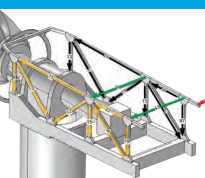
FIGURE 3: Calculated current distribution within the nacelle during a 200-kA lightning strike to the rear right corner of the nacelle. (All numbers refer to kA.)
